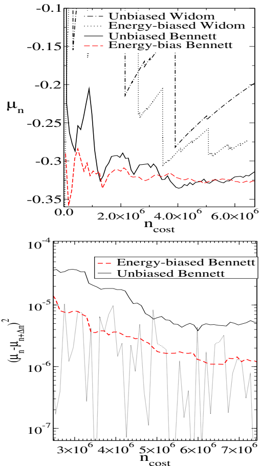
FIG. 2: (a) The estimation of the chemical potential plotted against the overall number of energy probes ( n_{cost} ). We compare the standard (uniform sampling) Bennett and Widom methods with the corresponding energy-biased versions of these methods. The calculations correspond to a Lennard-Jones fluid with \rho = 0.0236\text{\AA}^{-3} , and T = 84\text{K} ( \rho = 0.92\sigma^3 and T = 0.7\epsilon/k_B in reduced LJ units); the energy-biased sampling was done using u_w = 14.19 Kcal/mol and d = 15 samples per well. (b) The convergence measured as the squared difference between consecutive estimations with increasing cost ( \Delta n = 10^5 ). In the energy-biased method the cost is given by n_{cost} = n_0(1 + dF_w/a) , where n_0 is the number of random probes used to evaluate F_w(= F(u_w) = 0.00122) and a = 0.165 is the acceptance ratio of the Hit&Run sampler. Circles are the successive values of (\mu_n - \mu_{n+\Delta n})^2 (shown only for the energy-biased case) and solid lines are the average over twenty consecutive differences.
