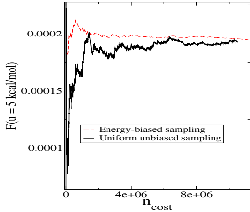
FIG. 4: The cumulative probability F(u) = \int_{-\infty}^u f(u') du' for u = 5 Kcal/mol versus the total number of energy evaluations of the test-particle n_{cost} . The liquid is the same as in Fig. 2. We compare the estimations of F(u) for grid-sampling (with a regular mesh of 36^3 nodes) and for energy-biased samplings within u < u_w = 14.19 Kcal/mol, performing d = 15 samples per well. The cumulative probability at u_w is F_w = F(u_w) = 0.00122 .
