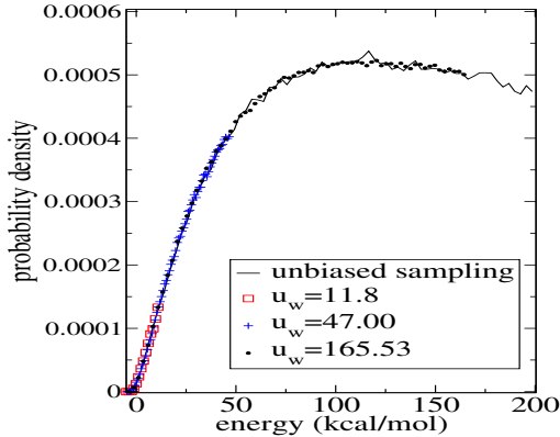
FIG. 3: The energy distribution f(u) obtained from 4 \times 10^6 random insertions over the whole configurational domain is compared with energy-biased sampling in the restricted configurational space u < u_w . The calculations correspond to the same case as in Fig. 2. The energy cavities are sampled using the Hit&Run algorithm, which provides an unbiased reconstruction of the energy distribution for any value of u_w chosen.
